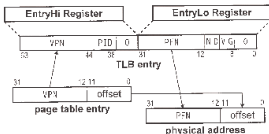
Figure 13-12. MIPS R3000 address translation.
